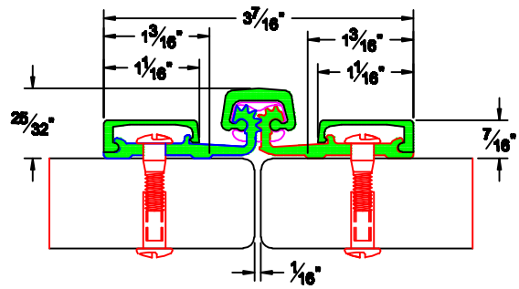
SL60/SL62 DOOR AND FRAME MOUNT FLUSH
