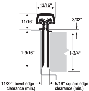
DOOR CLOSED
