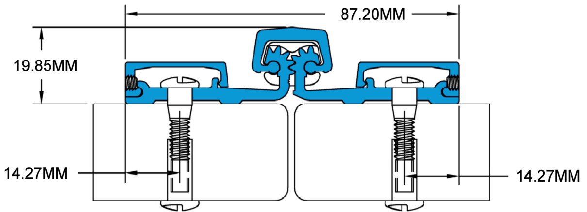
SL60/SL62 DOOR AND FRAME MOUNT FLUSH
